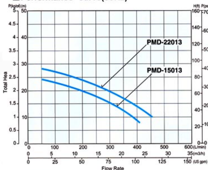
■ Performance curve(50Hz)
