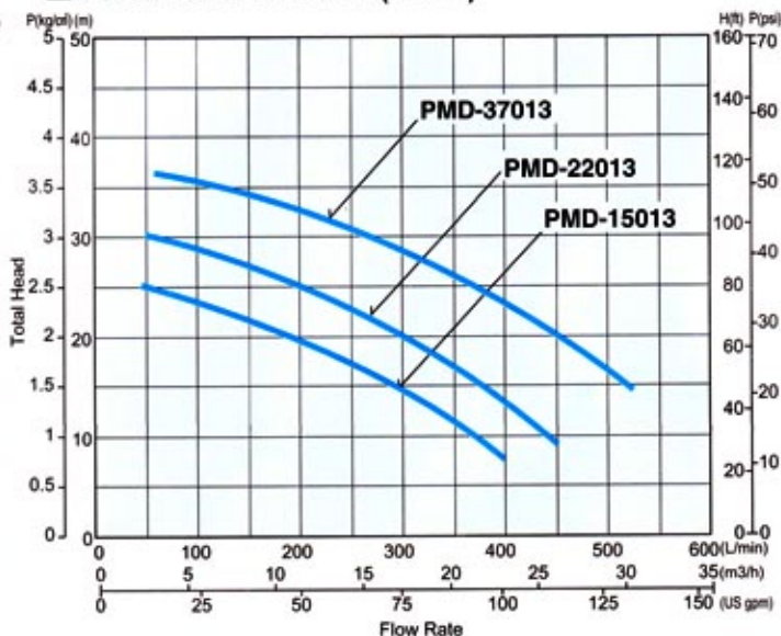
■ Performance curve(60Hz)
